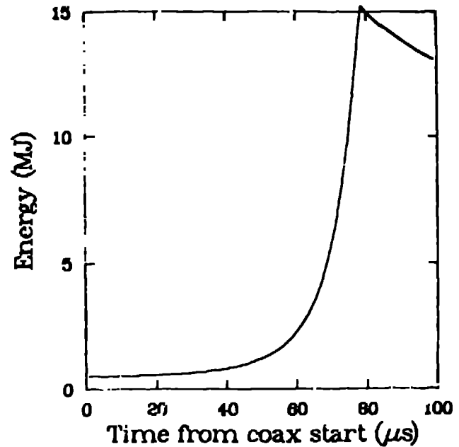
Fig. 5. Energy delivered to the 12.5 nH load in the high-power shot. The curve is calculated from LI^2/2 .
